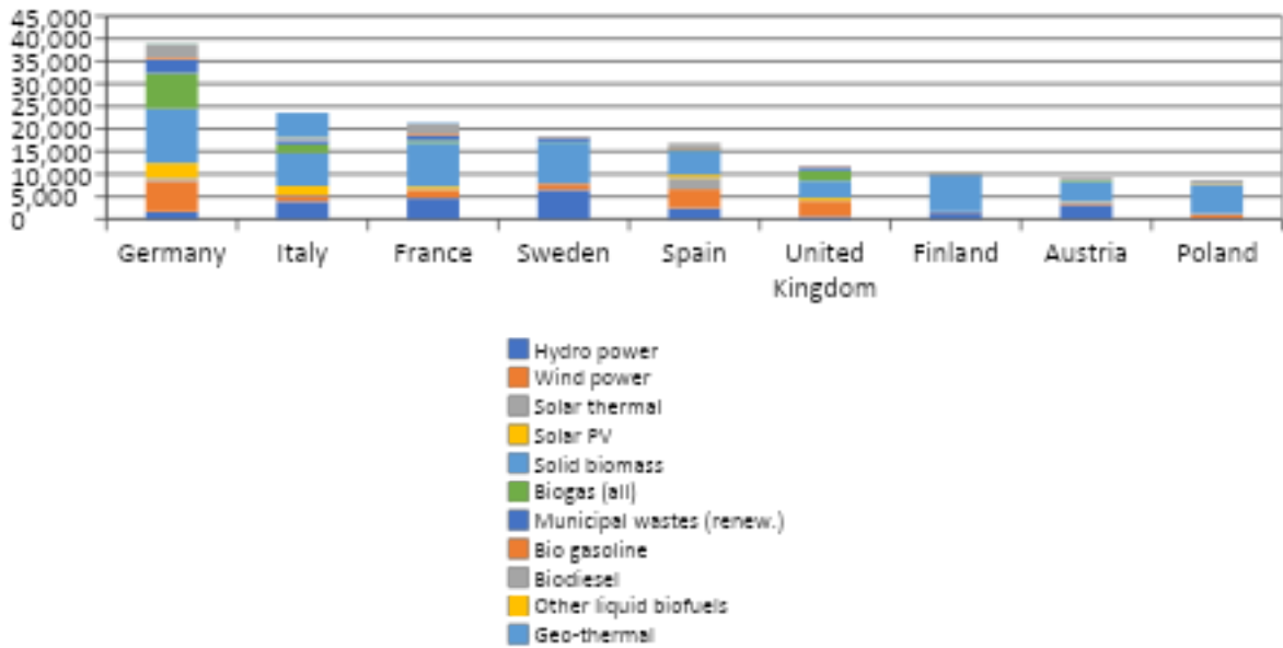
Fig. 5. The structure of RES used in the selected countries
